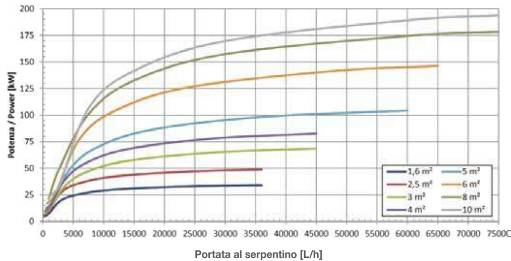
Potenza scambiata T_{in,coil} = 60\text{ }^{\circ}\text{C} ; T_{serb,in} = 10\text{ }^{\circ}\text{C} ; T_{serb,ou} = 45\text{ }^{\circ}\text{C}
