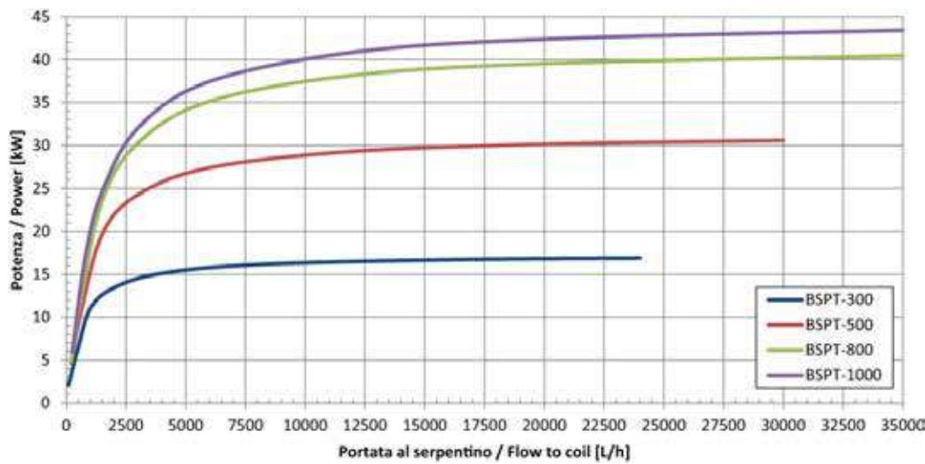
Potenza scambiata, scamb. PdC T_{in,coil} = 60\text{ }^{\circ}\text{C} ; T_{serb,in} = 10\text{ }^{\circ}\text{C} , T_{serb,out} = 45\text{ }^{\circ}\text{C}
