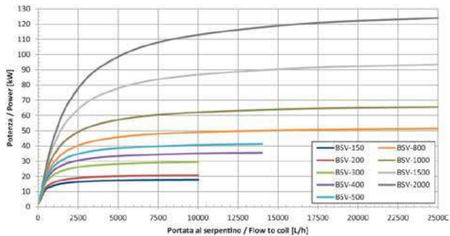
Potenza scambiata T_{in,coil} = 80\text{ }^{\circ}\text{C} ; T_{serb,in} = 10\text{ }^{\circ}\text{C} , T_{serb,out} = 45\text{ }^{\circ}\text{C}
