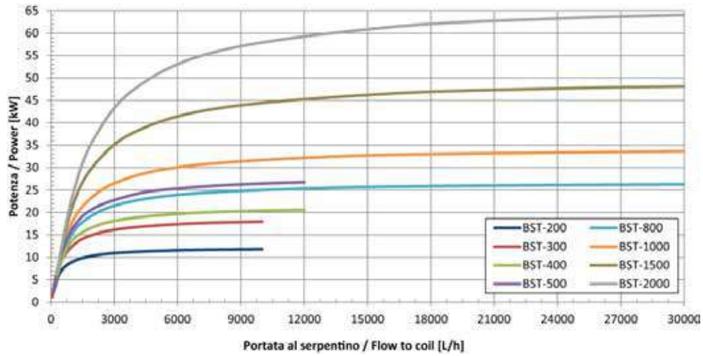
Potenza scambiata, scamb. solare T_{in,coil} = 60\text{ }^{\circ}\text{C} ; T_{serb,in} = 10\text{ }^{\circ}\text{C} , T_{serb,out} = 45\text{ }^{\circ}\text{C}
