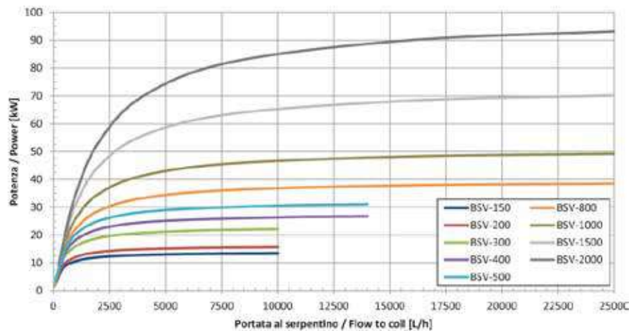
Potenza scambiata T_{in,coil} = 70\text{ }^{\circ}\text{C} ; T_{serb,in} = 10\text{ }^{\circ}\text{C} , T_{serb,out} = 45\text{ }^{\circ}\text{C}
