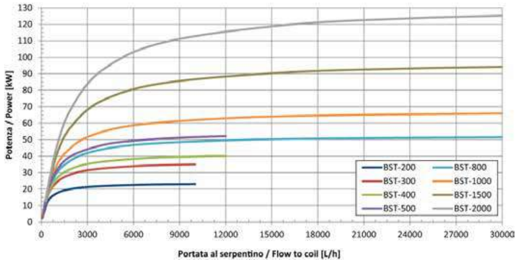
Potenza scambiata, scamb. solare T_{in,coil} = 80\text{ }^{\circ}\text{C} ; T_{serb,in} = 10\text{ }^{\circ}\text{C} , T_{serb,out} = 45\text{ }^{\circ}\text{C}
