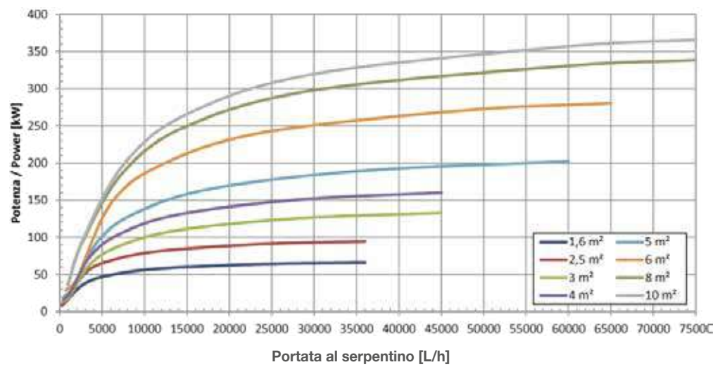
Potenza scambiata T_{in,coil} = 80\text{ }^{\circ}\text{C} ; T_{serb,in} = 10\text{ }^{\circ}\text{C} ; T_{serb,ou} = 45\text{ }^{\circ}\text{C}
