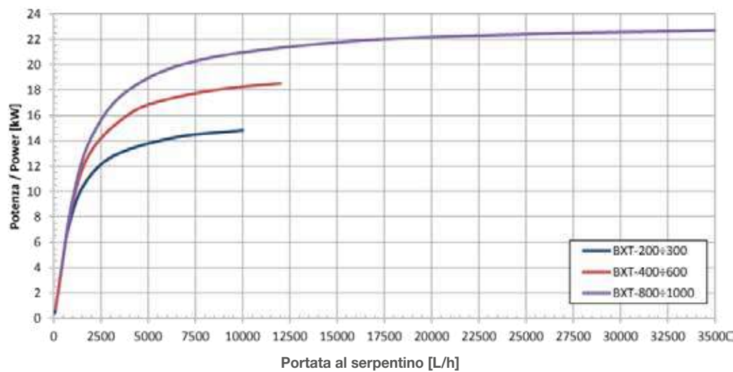
Potenza scambiata, scamb.integr. T_{in,coil} = 50\text{ }^{\circ}\text{C} ; T_{serb,in} = 10\text{ }^{\circ}\text{C} , T_{serb,out} = 45\text{ }^{\circ}\text{C}
