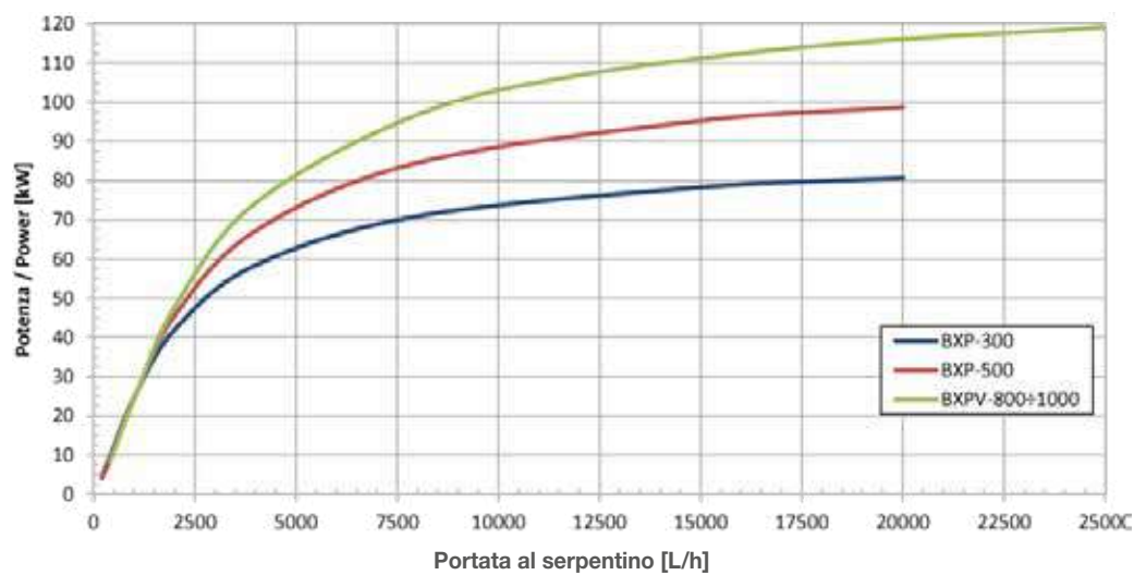
Potenza scambiata T_{in,coil} = 50\text{ }^{\circ}\text{C} ; T_{serb,in} = 10\text{ }^{\circ}\text{C} , T_{serb,out} = 45\text{ }^{\circ}\text{C}
