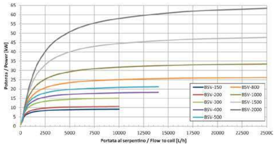
Potenza scambiata T_{in,coil} = 60\text{ }^{\circ}\text{C} ; T_{serb,in} = 10\text{ }^{\circ}\text{C} , T_{serb,out} = 45\text{ }^{\circ}\text{C}
