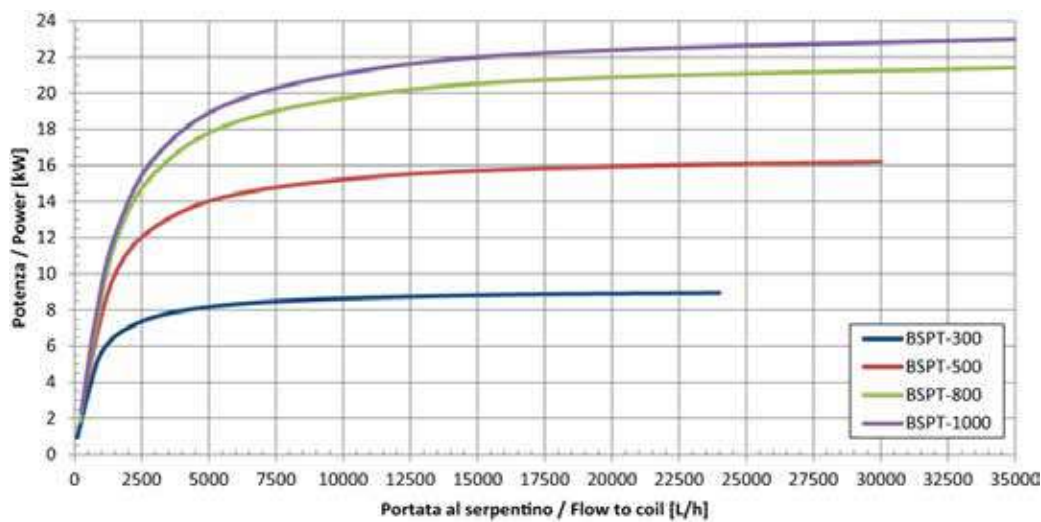
Potenza scambiata, scamb. PdC T_{in,coil} = 50\text{ }^{\circ}\text{C} ; T_{serb,in} = 10\text{ }^{\circ}\text{C} , T_{serb,out} = 45\text{ }^{\circ}\text{C}
