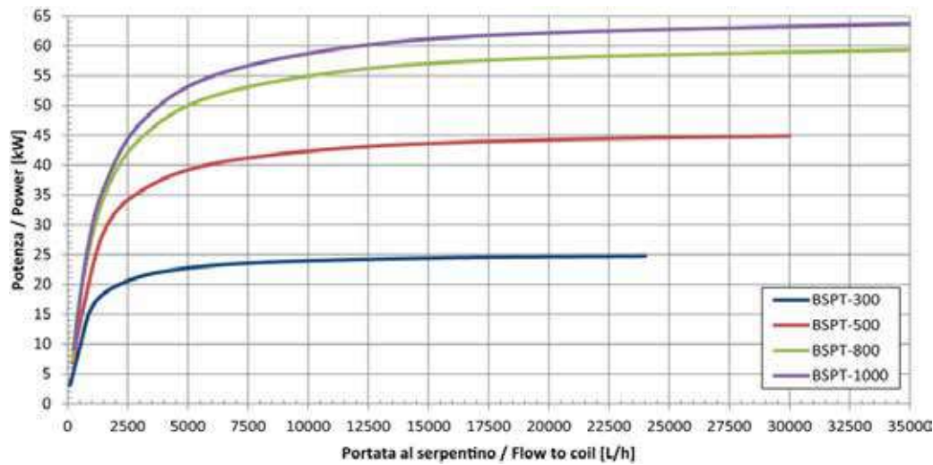
Potenza scambiata, scamb. PdC T_{in,coil} = 70\text{ }^{\circ}\text{C} ; T_{serb,in} = 10\text{ }^{\circ}\text{C} , T_{serb,out} = 45\text{ }^{\circ}\text{C}
