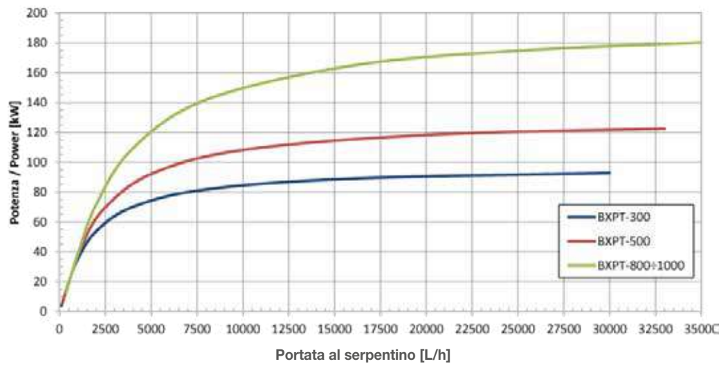
Potenza scambiata, scamb. PdC T_{in,coil} = 60\text{ }^{\circ}\text{C} ; T_{serb,in} = 10\text{ }^{\circ}\text{C} , T_{serb,out} = 45\text{ }^{\circ}\text{C}
