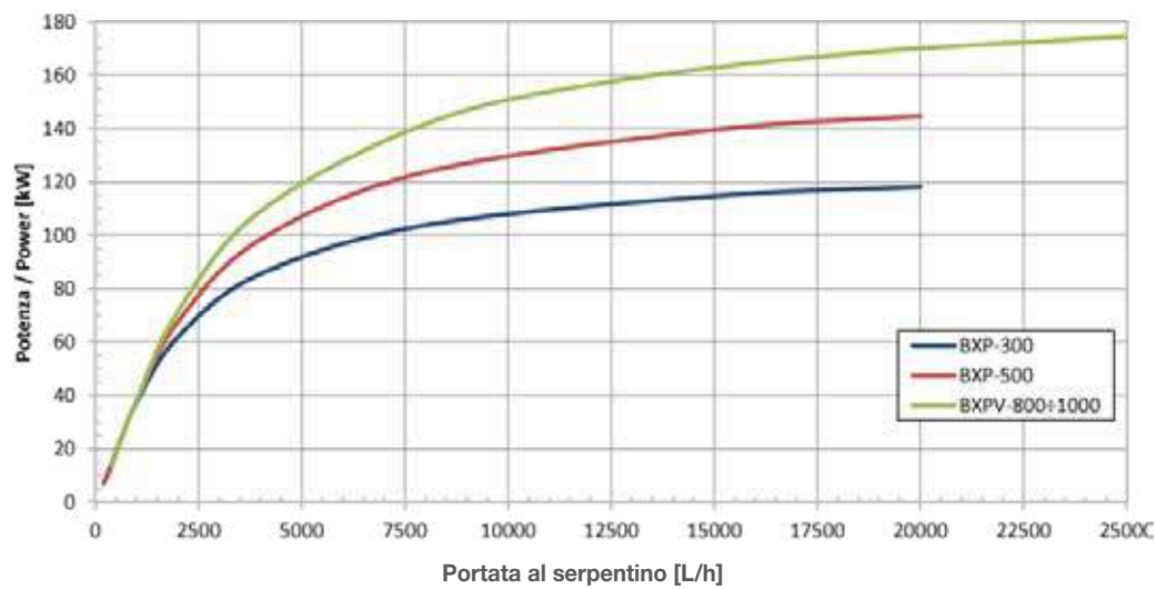
Potenza scambiata T_{in,coil} = 60\text{ }^{\circ}\text{C} ; T_{serb,in} = 10\text{ }^{\circ}\text{C} , T_{serb,out} = 45\text{ }^{\circ}\text{C}
