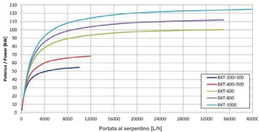
Potenza scambiata, scamb. solare T_{in,coil} = 70\text{ }^{\circ}\text{C} ; T_{serb,in} = 10\text{ }^{\circ}\text{C} , T_{serb,out} = 45\text{ }^{\circ}\text{C}
