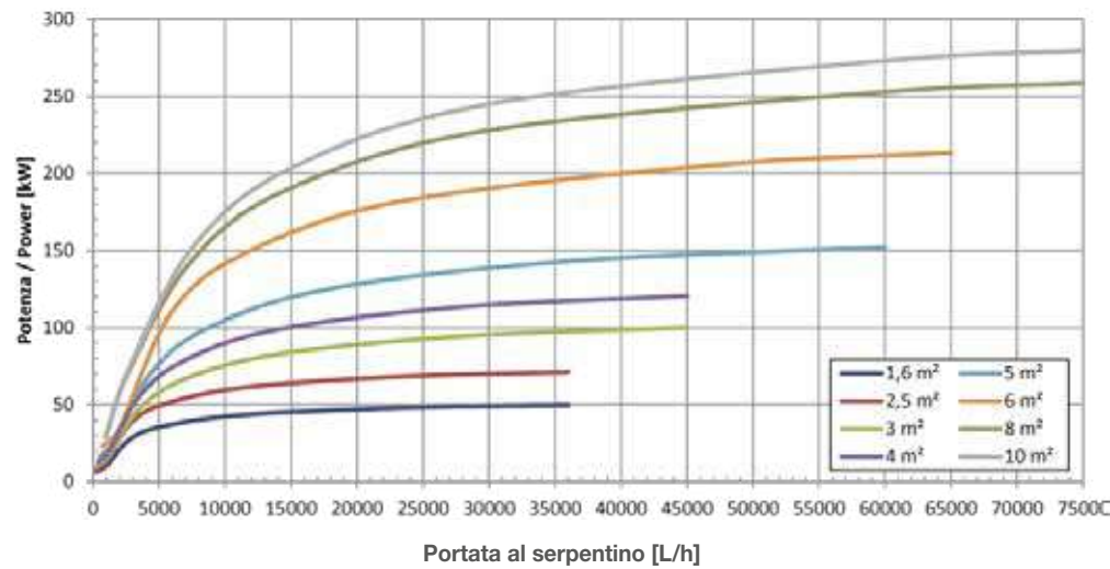
Potenza scambiata T_{in,coil} = 70\text{ }^{\circ}\text{C} ; T_{serb,in} = 10\text{ }^{\circ}\text{C} ; T_{serb,ou} = 45\text{ }^{\circ}\text{C}
